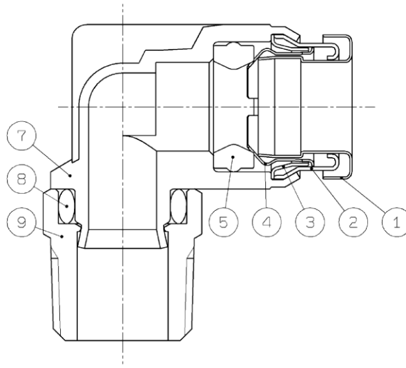
Male elbow
