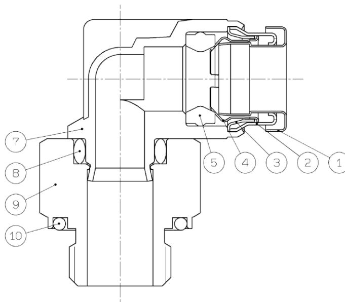
Male elbow
